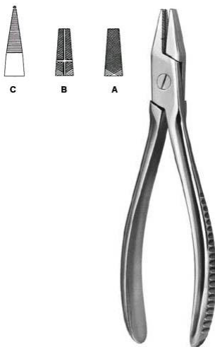
AS-7-120-01 Flat Nose Plier 17.5 cm,
