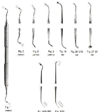
Westcott AS-65-101 Filling instruments Fig- 1,
